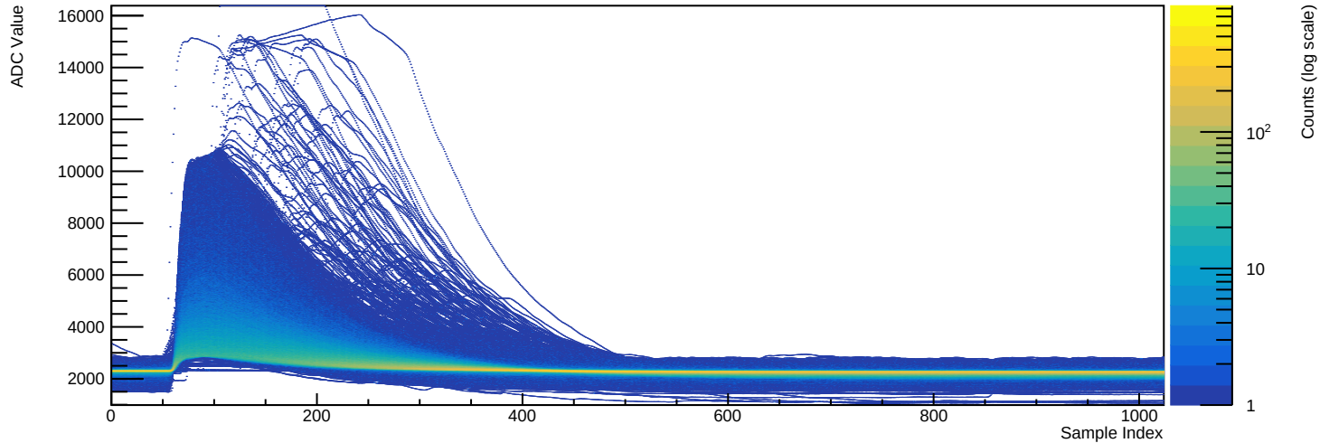
Run 039518 - Channel 2081 (n=29657 waveforms)
