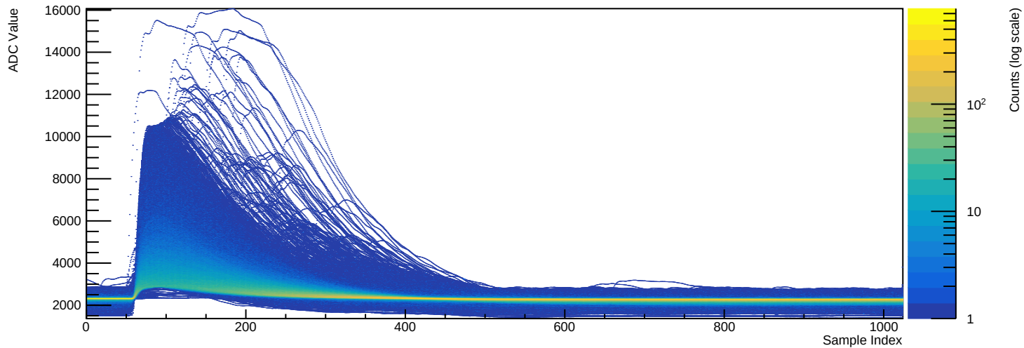
Run 039522 - Channel 2081 (n=27141 waveforms)
