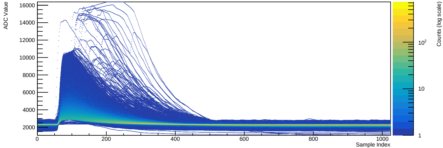
Run 039529 - Channel 2081 (n=23747 waveforms)
