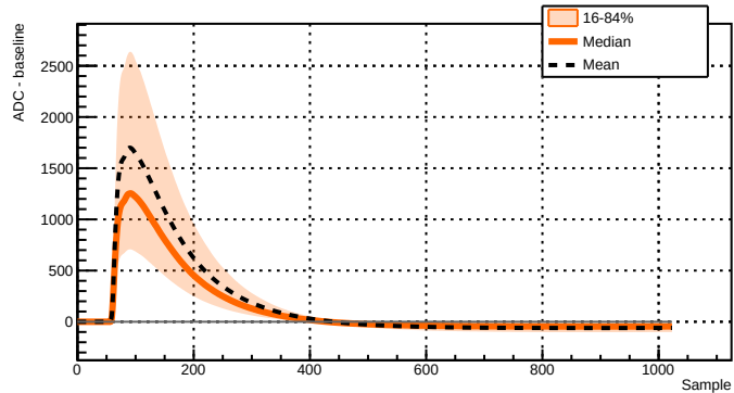
Run 039500 - Channel 2081 - 24447 waveforms
