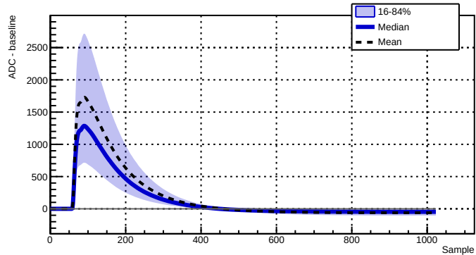
Run 039500 - Channel 2080 - 24911 waveforms
