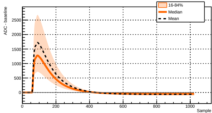
Run 039501 - Channel 2081 - 25227 waveforms
