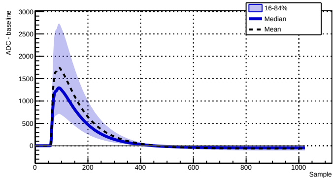
Run 039501 - Channel 2080 - 25816 waveforms
