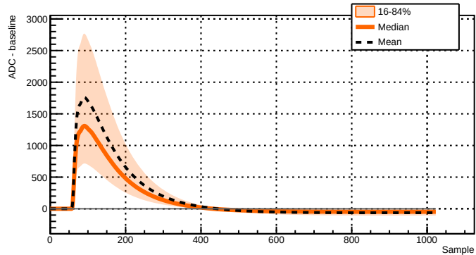
Run 039502 - Channel 2081 - 26350 waveforms
