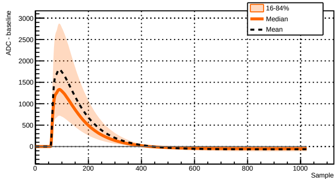
Run 039503 - Channel 2081 - 27934 waveforms
