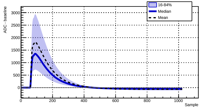
Run 039503 - Channel 2080 - 28528 waveforms
