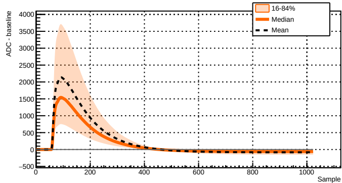
Run 039510 - Channel 2081 - 38133 waveforms
