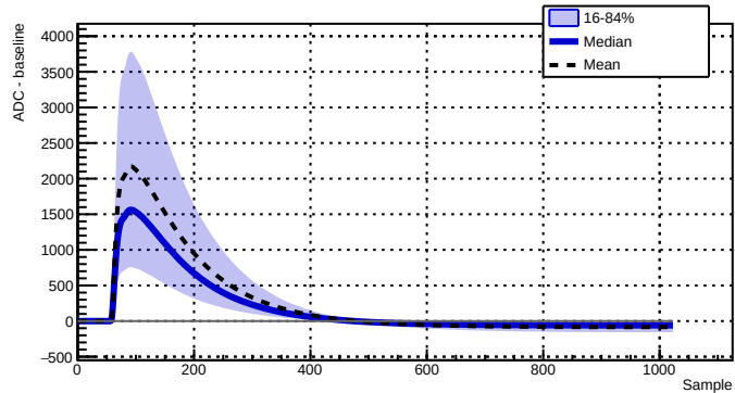
Run 039510 - Channel 2080 - 38593 waveforms
