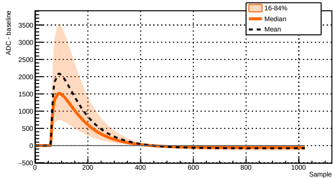
Run 039512 - Channel 2081 - 35084 waveforms
