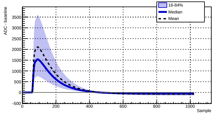
Run 039512 - Channel 2080 - 35509 waveforms
