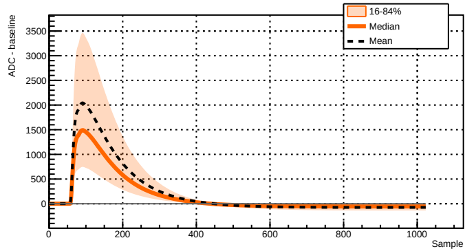
Run 039514 - Channel 2081 - 33359 waveforms
