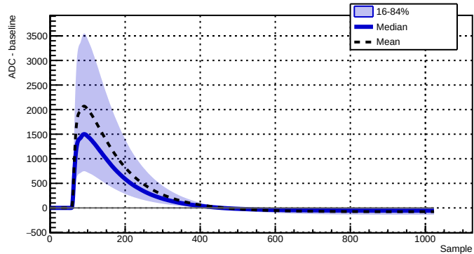
Run 039514 - Channel 2080 - 33915 waveforms
