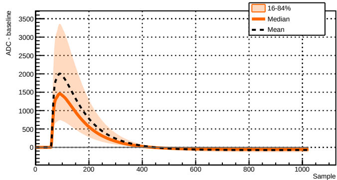
Run 039515 - Channel 2081 - 31555 waveforms
