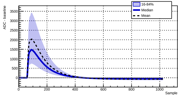
Run 039515 - Channel 2080 - 32102 waveforms
