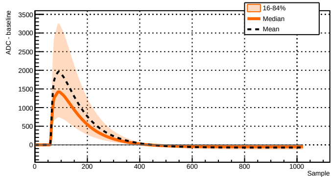
Run 039516 - Channel 2081 - 30535 waveforms
