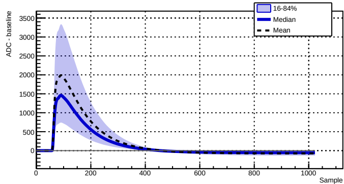
Run 039516 - Channel 2080 - 30954 waveforms
