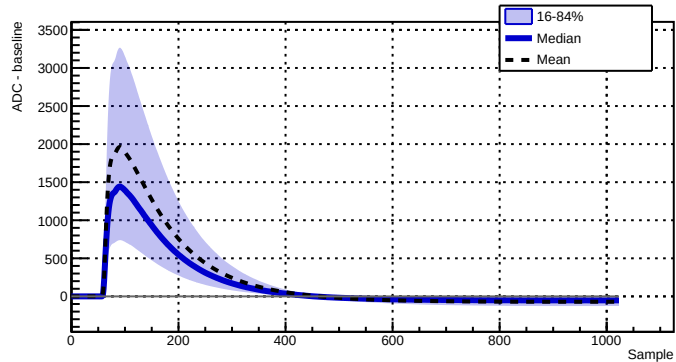
Run 039517 - Channel 2080 - 30921 waveforms
