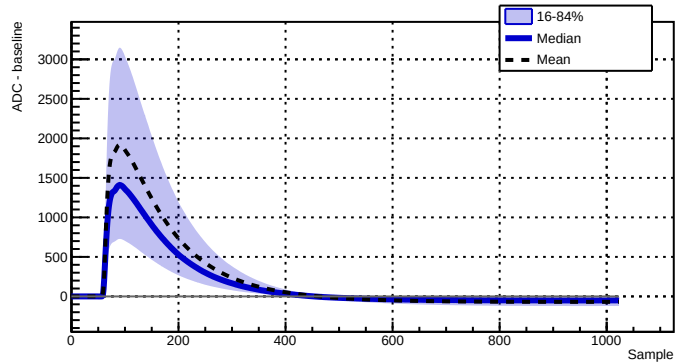
Run 039518 - Channel 2080 - 30238 waveforms
