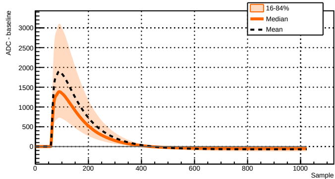
Run 039518 - Channel 2081 - 29657 waveforms
