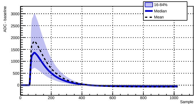
Run 039521 - Channel 2080 - 28127 waveforms
