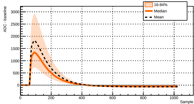
Run 039521 - Channel 2081 - 27619 waveforms
