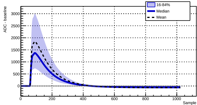
Run 039522 - Channel 2080 - 27597 waveforms
