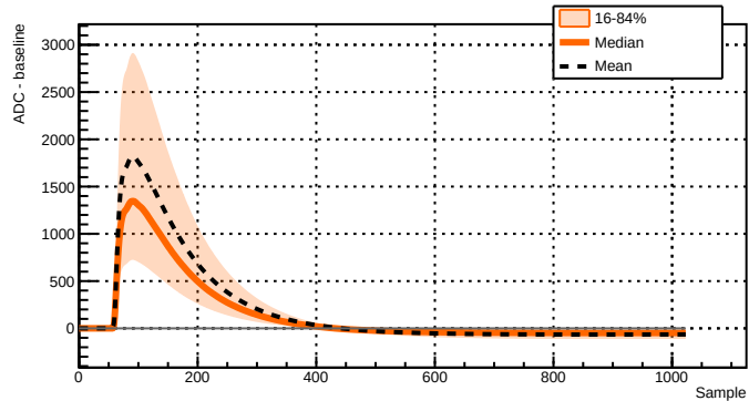
Run 039522 - Channel 2081 - 27141 waveforms
