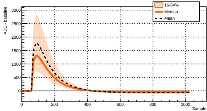
Run 039523 - Channel 2081 - 26250 waveforms
