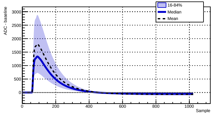
Run 039523 - Channel 2080 - 26712 waveforms
