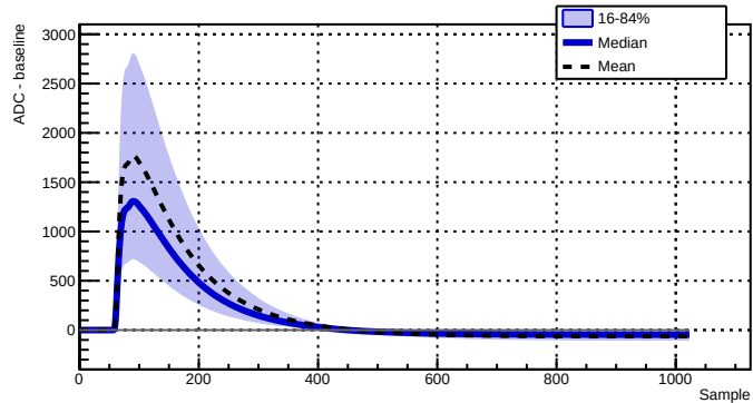
Run 039526 - Channel 2080 - 25571 waveforms
