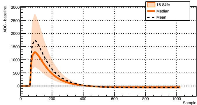
Run 039526 - Channel 2081 - 25159 waveforms
