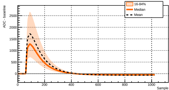
Run 039527 - Channel 2081 - 24637 waveforms
