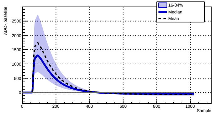
Run 039527 - Channel 2080 - 25215 waveforms
