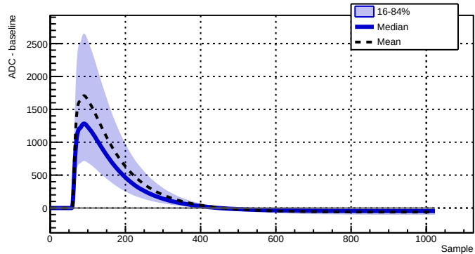
Run 039529 - Channel 2080 - 24240 waveforms
