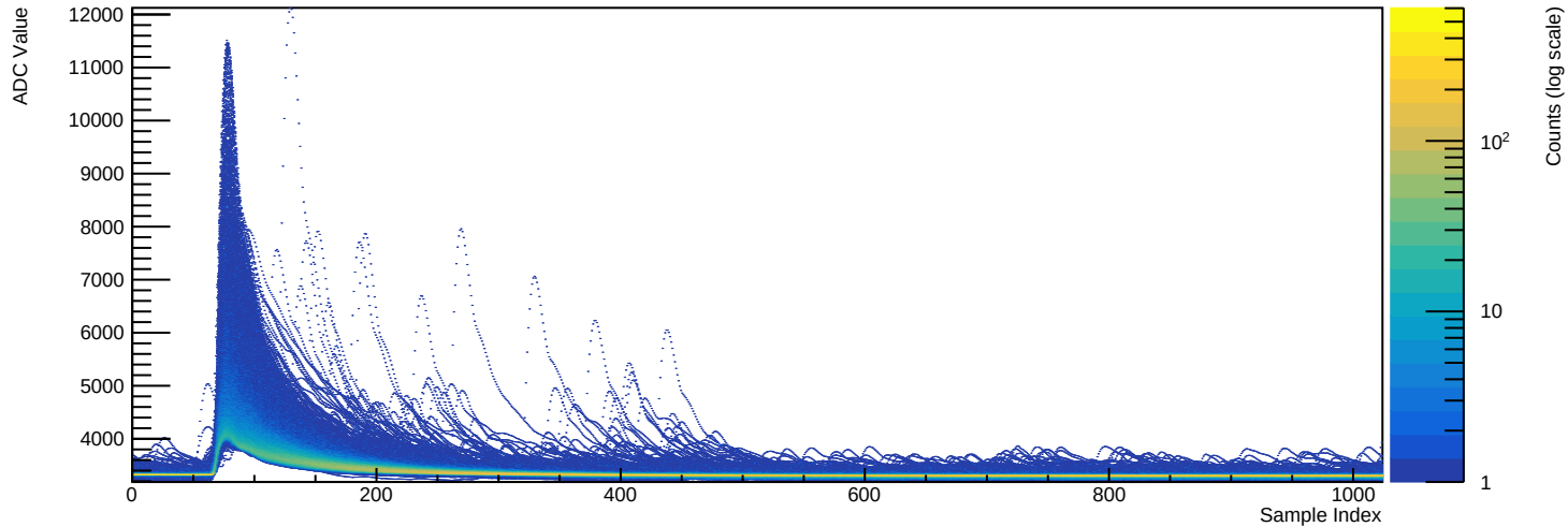
Run 039501 - Channel 2070 (n=9678 waveforms)
