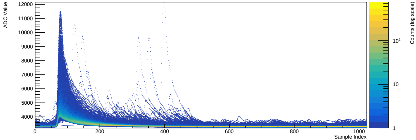
Run 039506 - Channel 2070 (n=13239 waveforms)
