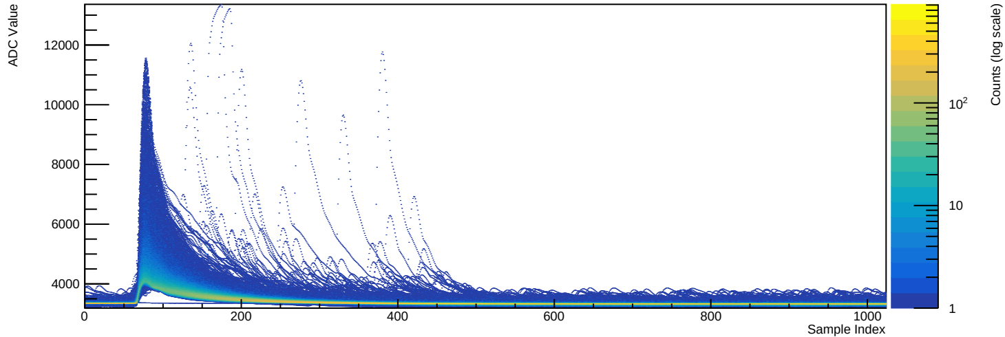
Run 039512 - Channel 2070 (n=16659 waveforms)
