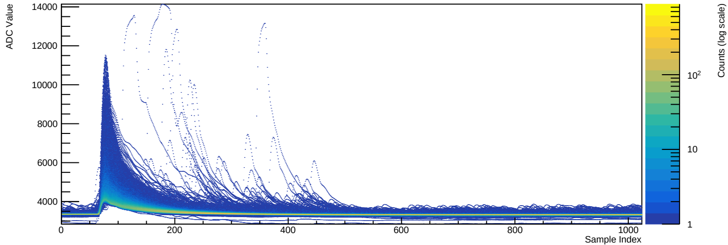
Run 039514 - Channel 2070 (n=15376 waveforms)
