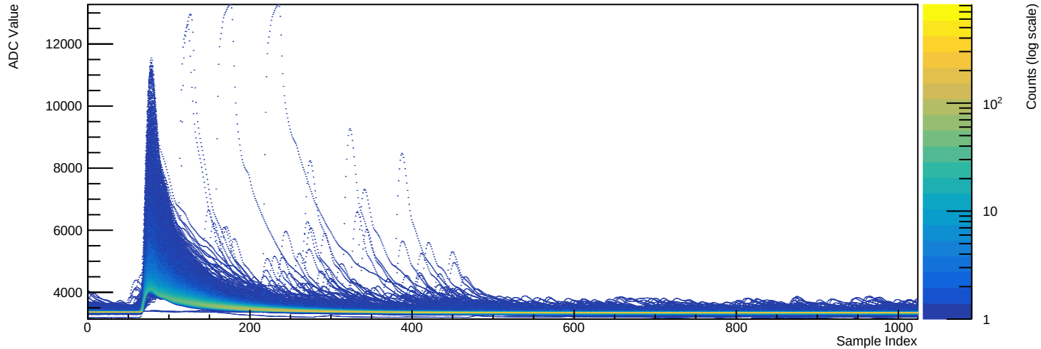
Run 039518 - Channel 2070 (n=12482 waveforms)
