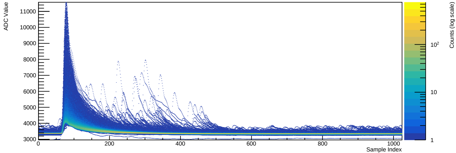
Run 039519 - Channel 2070 (n=12009 waveforms)
