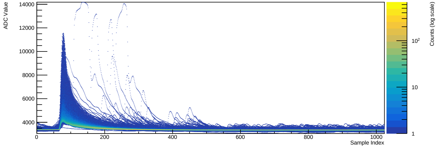
Run 039522 - Channel 2070 (n=11002 waveforms)
