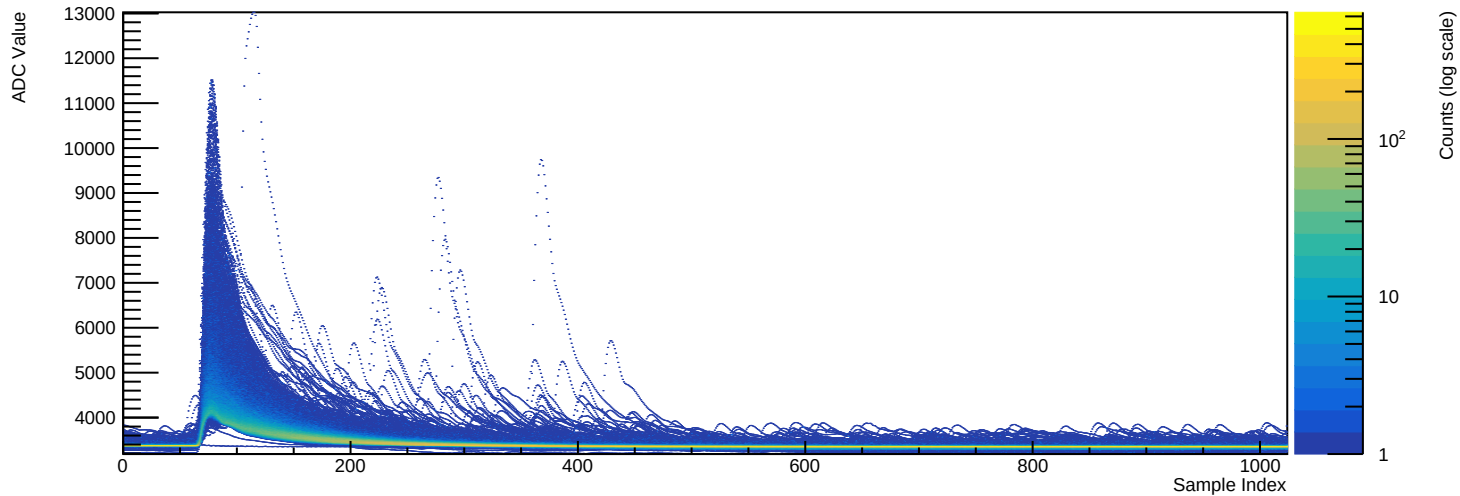
Run 039525 - Channel 2070 (n=10069 waveforms)
