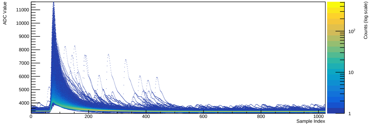
Run 039501 - Channel 2071 (n=9232 waveforms)
