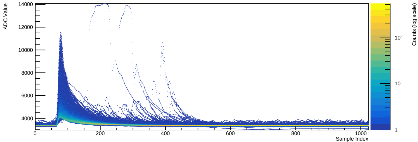
Run 039502 - Channel 2071 (n=9912 waveforms)
