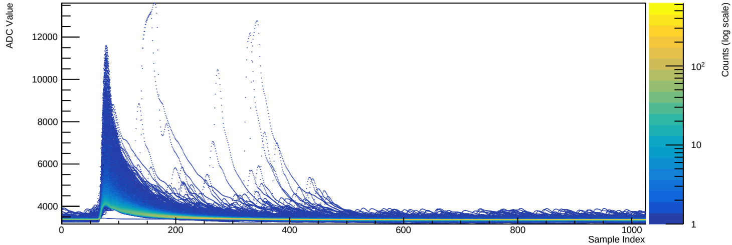
Run 039503 - Channel 2071 (n=10874 waveforms)
