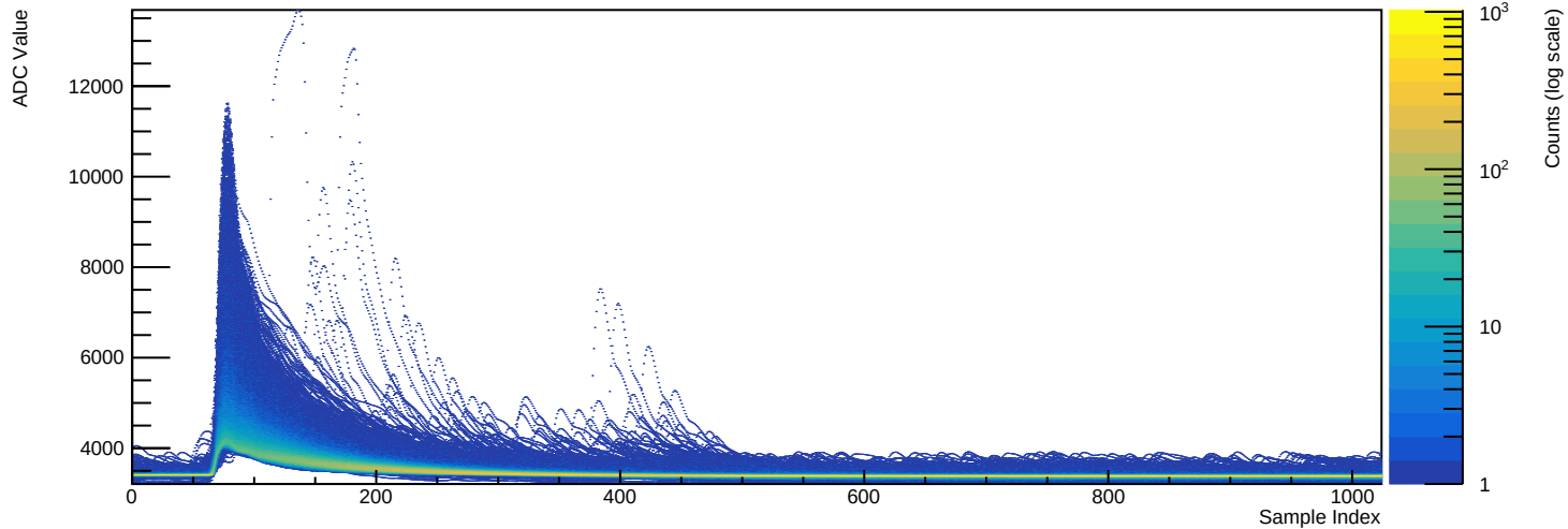
Run 039510 - Channel 2071 (n=18503 waveforms)
