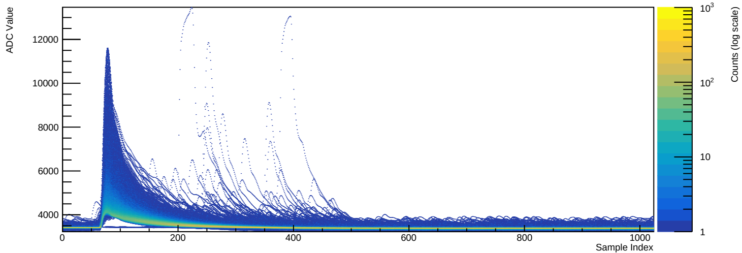
Run 039511 - Channel 2071 (n=17632 waveforms)
