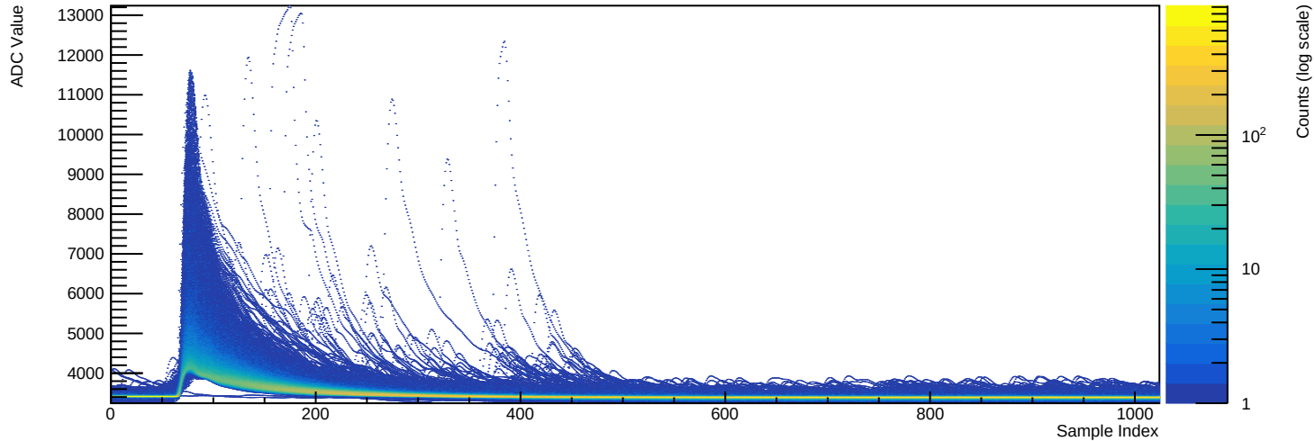
Run 039512 - Channel 2071 (n=16126 waveforms)
