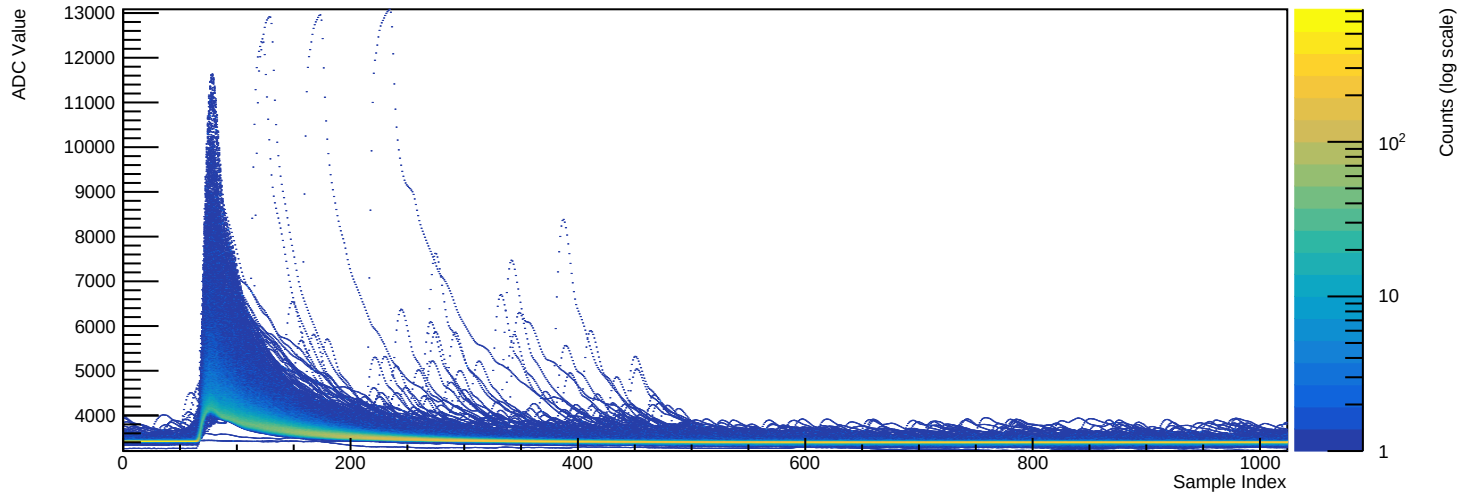
Run 039518 - Channel 2071 (n=12122 waveforms)
