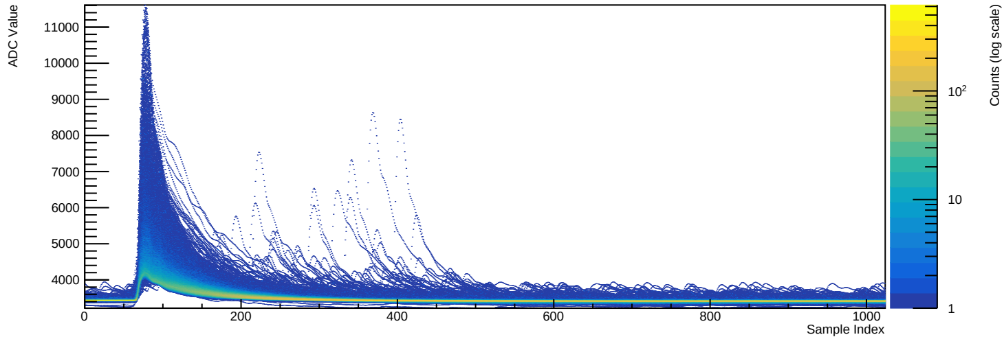
Run 039521 - Channel 2071 (n=10859 waveforms)
