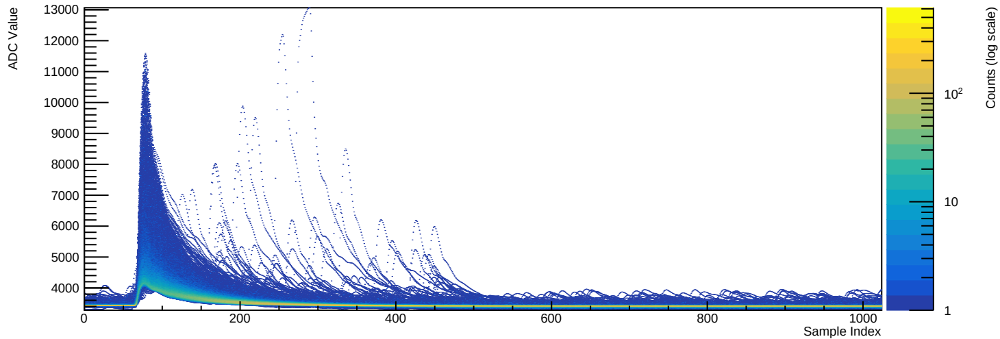
Run 039523 - Channel 2071 (n=10027 waveforms)
