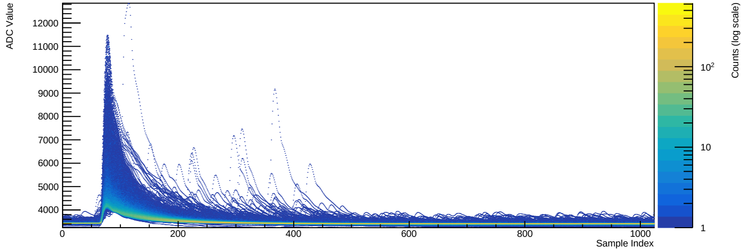
Run 039525 - Channel 2071 (n=9793 waveforms)
