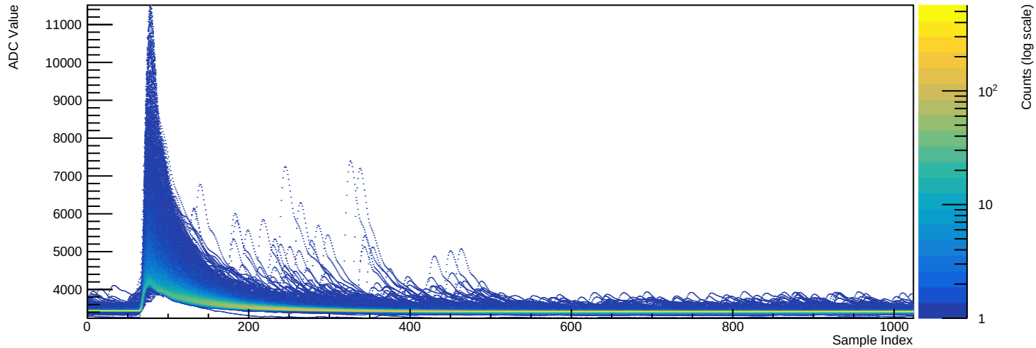
Run 039526 - Channel 2071 (n=9480 waveforms)
