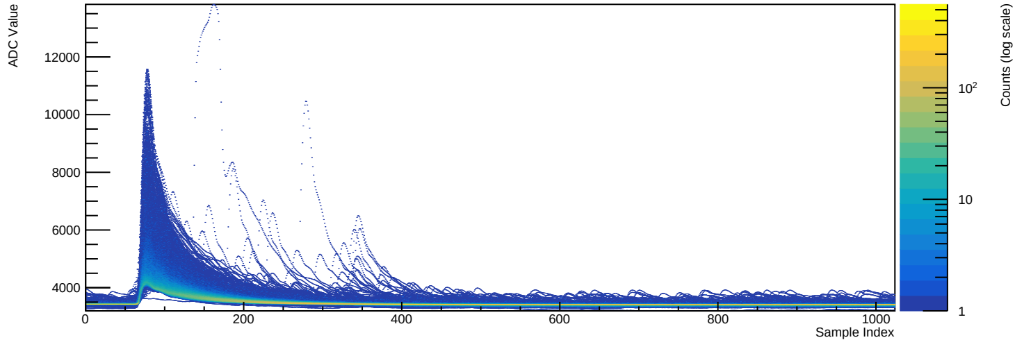
Run 039528 - Channel 2071 (n=8953 waveforms)
