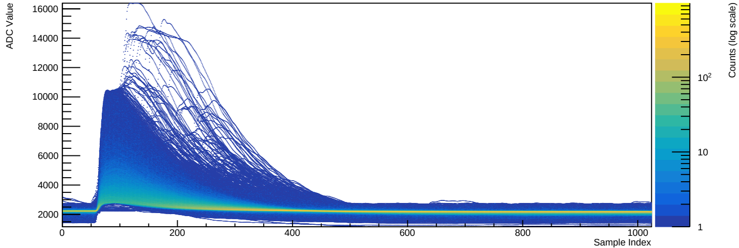
Run 039500 - Channel 2080 (n=32054 waveforms)
