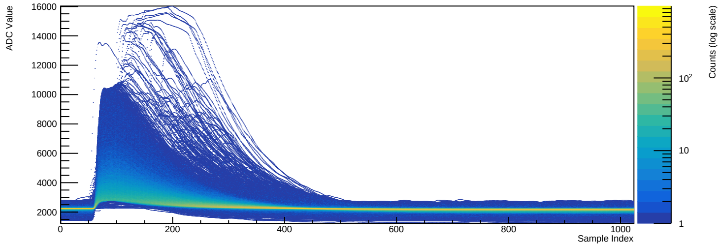
Run 039501 - Channel 2080 (n=33111 waveforms)
