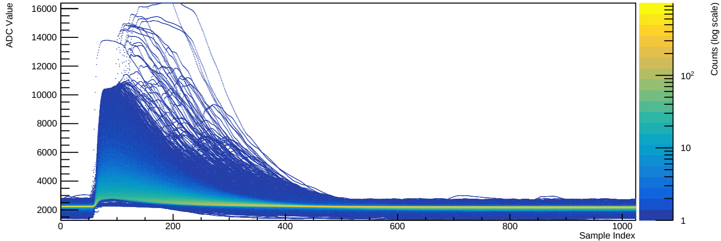
Run 039502 - Channel 2080 (n=34159 waveforms)
