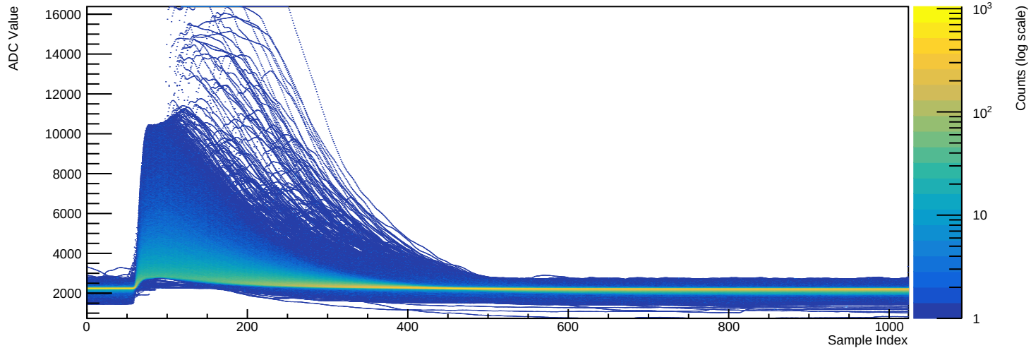
Run 039504 - Channel 2080 (n=37342 waveforms)
