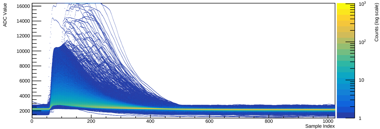
Run 039506 - Channel 2080 (n=39554 waveforms)
