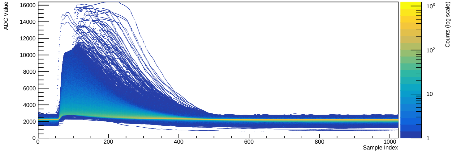
Run 039510 - Channel 2080 (n=48059 waveforms)
