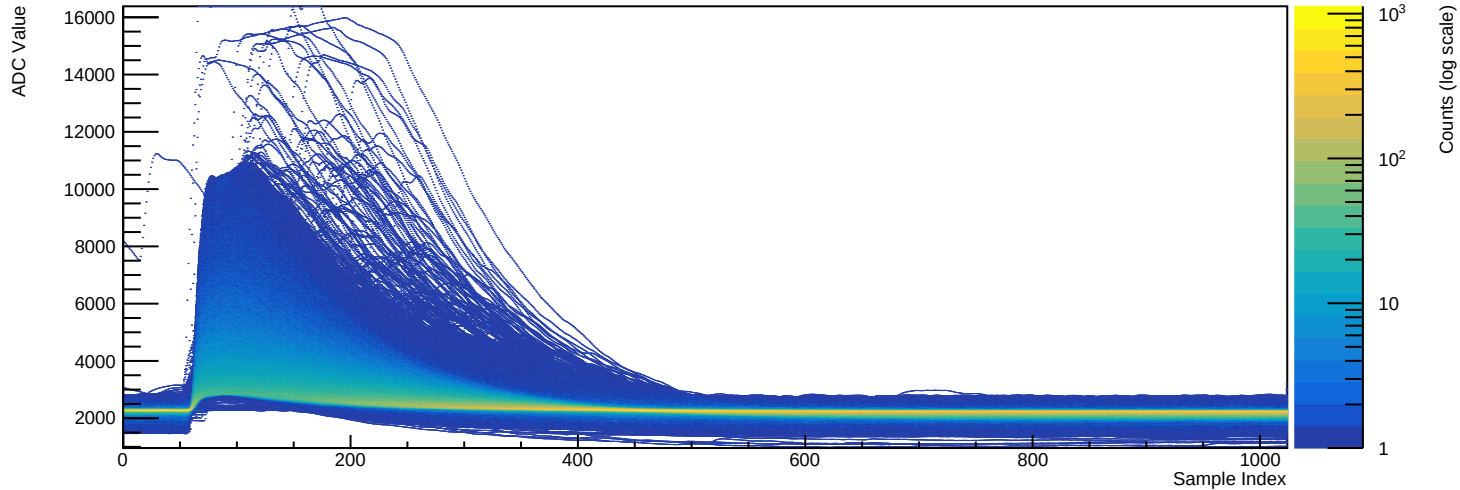
Run 039512 - Channel 2080 (n=44454 waveforms)
