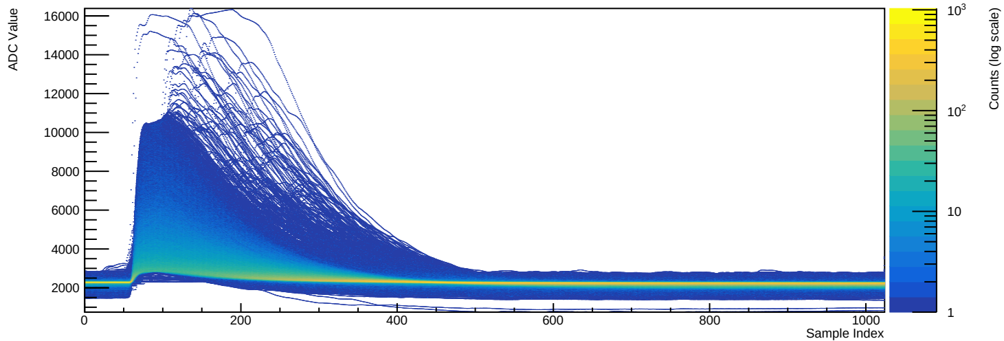
Run 039515 - Channel 2080 (n=40436 waveforms)
