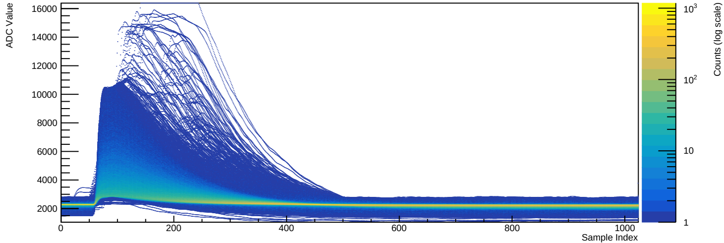
Run 039516 - Channel 2080 (n=39237 waveforms)
