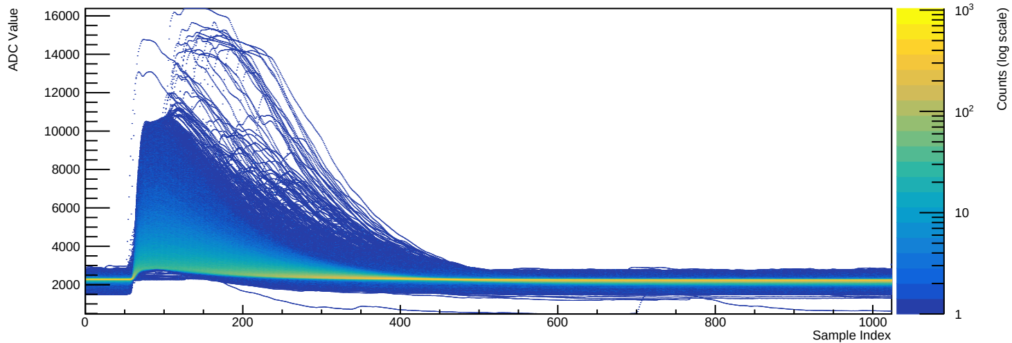
Run 039517 - Channel 2080 (n=39067 waveforms)
